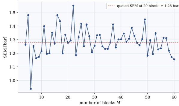
Figure 3: (b) Standard error of the mean pressure at \rho^* = 0.05 versus the number of blocks M . The SEM shows no systematic drift with M , confirming the blocks are long compared with the pressure correlation time and that the quoted \pm 1.28 \text{ bar} (dashed, at M = 20 ) is not an artefact of the block count.
