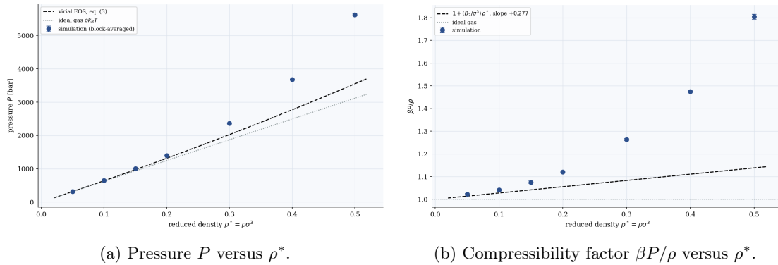
Figure 4: (c) Measured EOS (block-averaged points) versus the two-term virial prediction (dashed) and the ideal gas (dotted). (a) Pressure in bar. (b) Compressibility factor: the data follow the predicted slope B_2/\sigma^3 = +0.277 only at low density and then curve upward as higher-order virial terms become important. The truncated EOS holds up to \rho^* \sim 0.1 and underestimates P thereafter.
