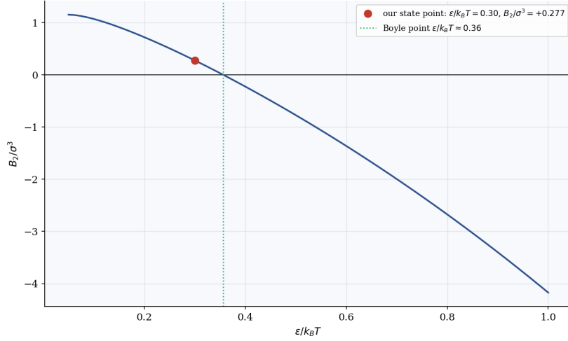
Figure 1: (a) Reduced second virial coefficient B_2/\sigma^3 versus \epsilon/k_B T for the shifted-cutoff LJ potential. The coefficient is positive at high temperature (repulsion-dominated), changes sign at the Boyle point \epsilon/k_B T \approx 0.356 (dotted), and turns negative at low temperature (attraction-dominated). The marker shows our state point, \epsilon/k_B T = 0.30 , B_2/\sigma^3 = +0.277 .
